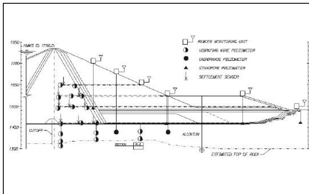
Figure 3. Typical distribution of the instruments in one of the dam cross
