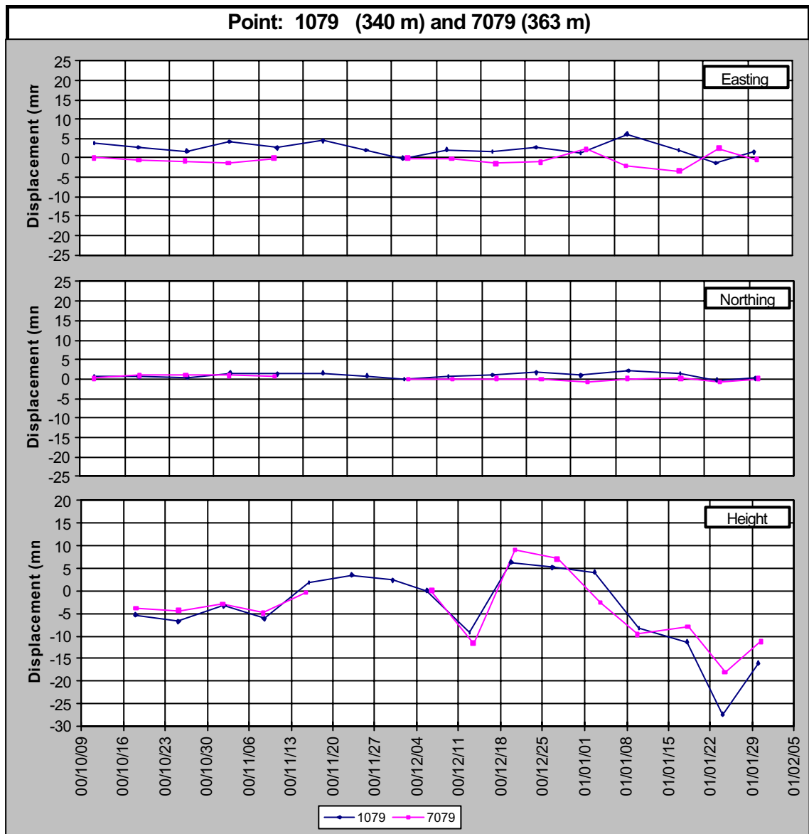
Figure 9. Displacement components for double point 1079/7079.
