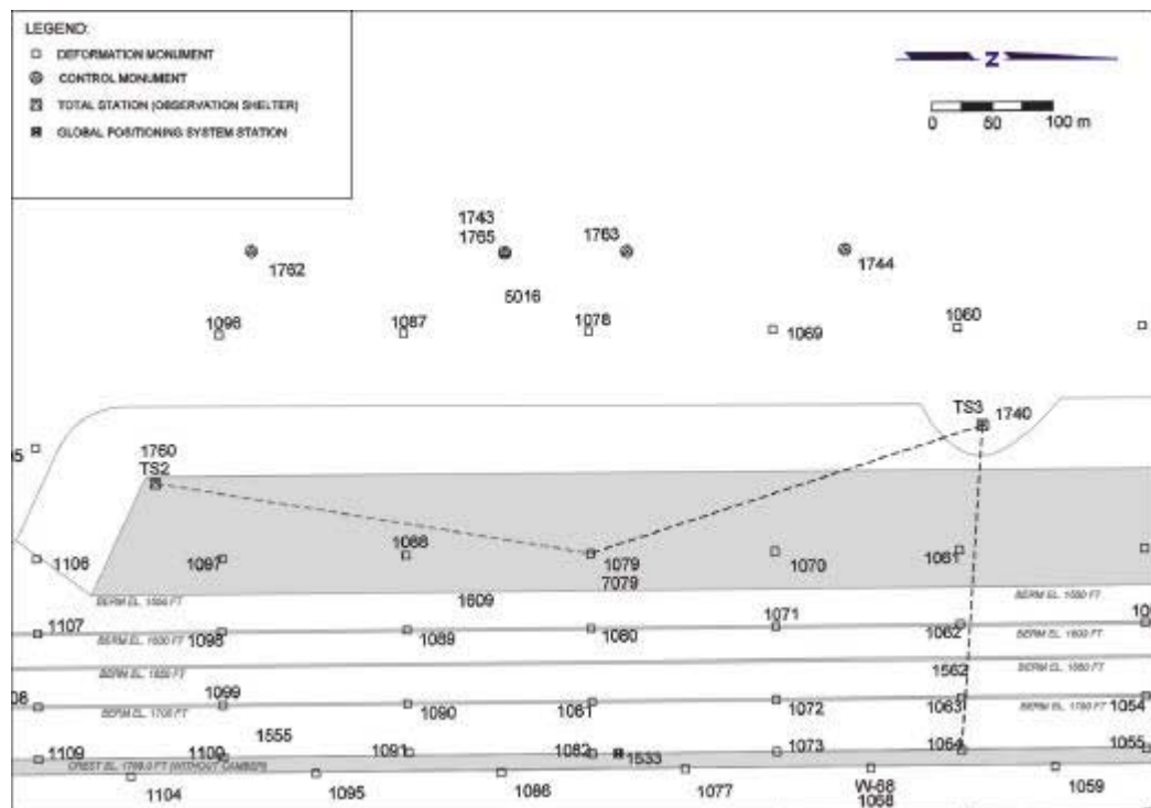
Figure 8. Example of a double-observed point.
