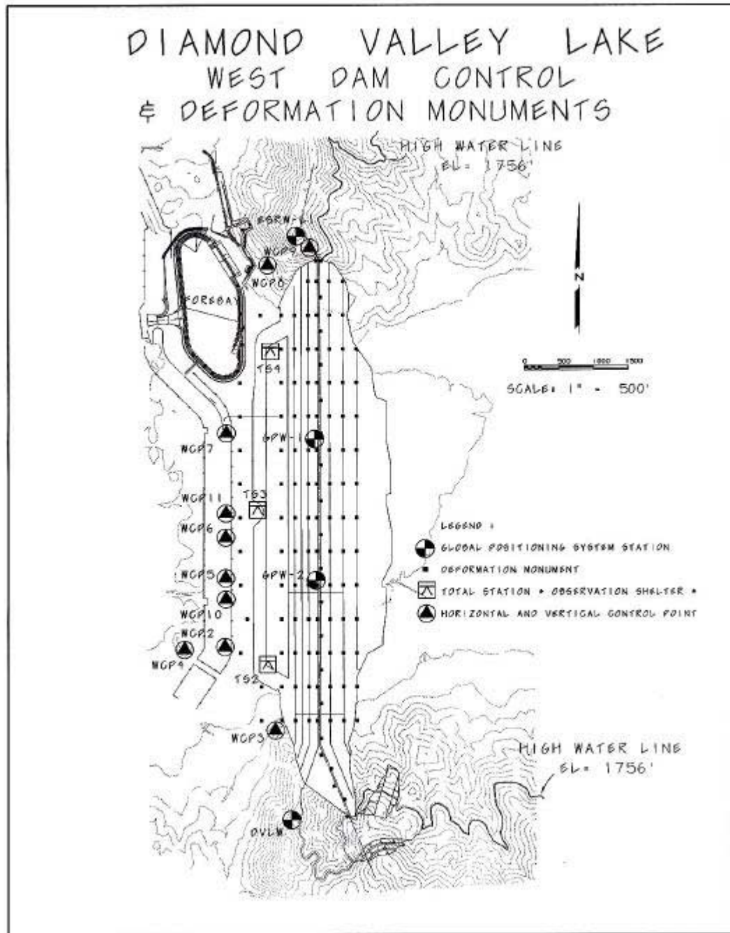
Figure 5. Observation scheme at the West Dam.
